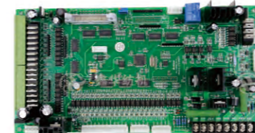
MOTHERBOARD (WEFT-SELECTING BOX)
