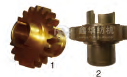
XH-S0548 Name: Weft Gear wheel No: BDY117A/BDY166A Notes:
