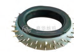
XH-S1824 Name: Temple ring (rubber) No: Notes: Three needle
