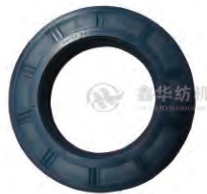
XH-S1033 Name: Oil seal No: VA12018 Notes: 55*90*10/8
