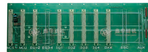
XH-S0094 Name: MOTHER BOARD Plate No: HULB-4B Notes:
