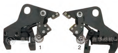
XH-S1316 Name: Selva cutter No: ALT201C/202C Notes: SM93
