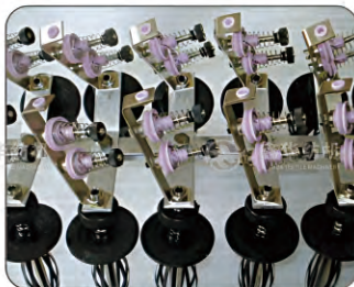
XH-S1886 Name: Scrap edge creel No: Notes:
