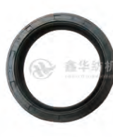
XH-S1034 Name: Oil seal No: VA11506 Notes: 55*72*8
