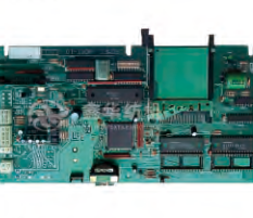
XH-S0020 Name: OPT-4A Circuit board No: A4E049A Notes:
