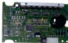
XH-S0273 Name: Weft Accumulator Board No: Notes:
