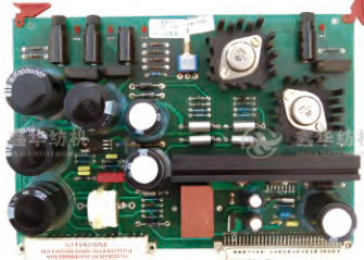
XH-V1727 Name: Breadboard No: Notes: 50H340
