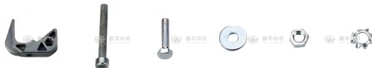
XH-V1304 Name: Seat of pressure No: 2556008 Notes: XH-V1305 Name: Bolt No: 0021017 Notes: M5*35 XH-V1306 Name: Bolt No: 0011006 Notes: M5*20 XH-V1307 Name: Flat gasket No: 0121002 Notes: Φ5.3 XH-V1308 Name: Nut No: 0101003 Notes: M5 XH-V1309 Name: Gasket No: 0131002 Notes: Φ5.1
