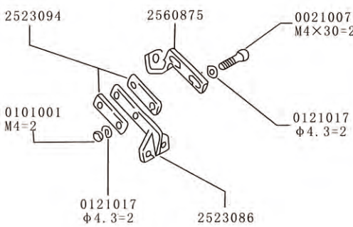
K88 Track support assembly 9120213
