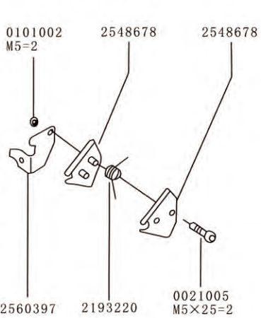
K88 Lubricating block seat assem 9120291
