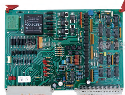
XH-V1726 Name: Breadboard No: Notes: D801
