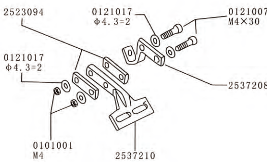
K88 Track support assembly(wide) 9120313
