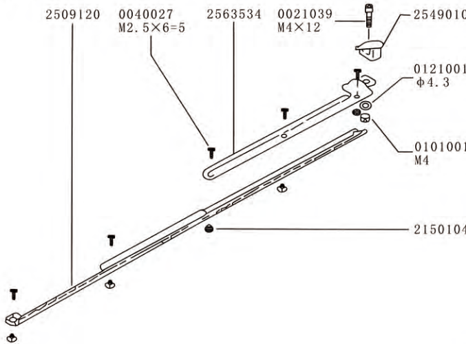
K88 Left guide bar assembly 9120373
