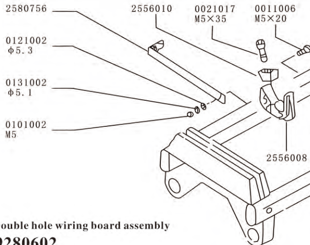
K88 Track support assembly 9120213
