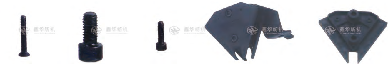
XH-V1493 Name: Screw No: 0042015 Notes: M6*40 XH-V1494 Name: Screw No: 0012004 Notes: M6*20 XH-V1495 Name: Screw No: 0021049 Notes: M5*10 XH-V1496 Name: Lubricating block seat No: 9120291 Notes: XH-V1497 Name: Box No: 2548678 Notes:
