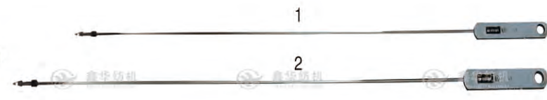
XH-V1697 Name: Lifting frame rod No: F19968610/F19968611 Notes: L1113mm/1153mm
